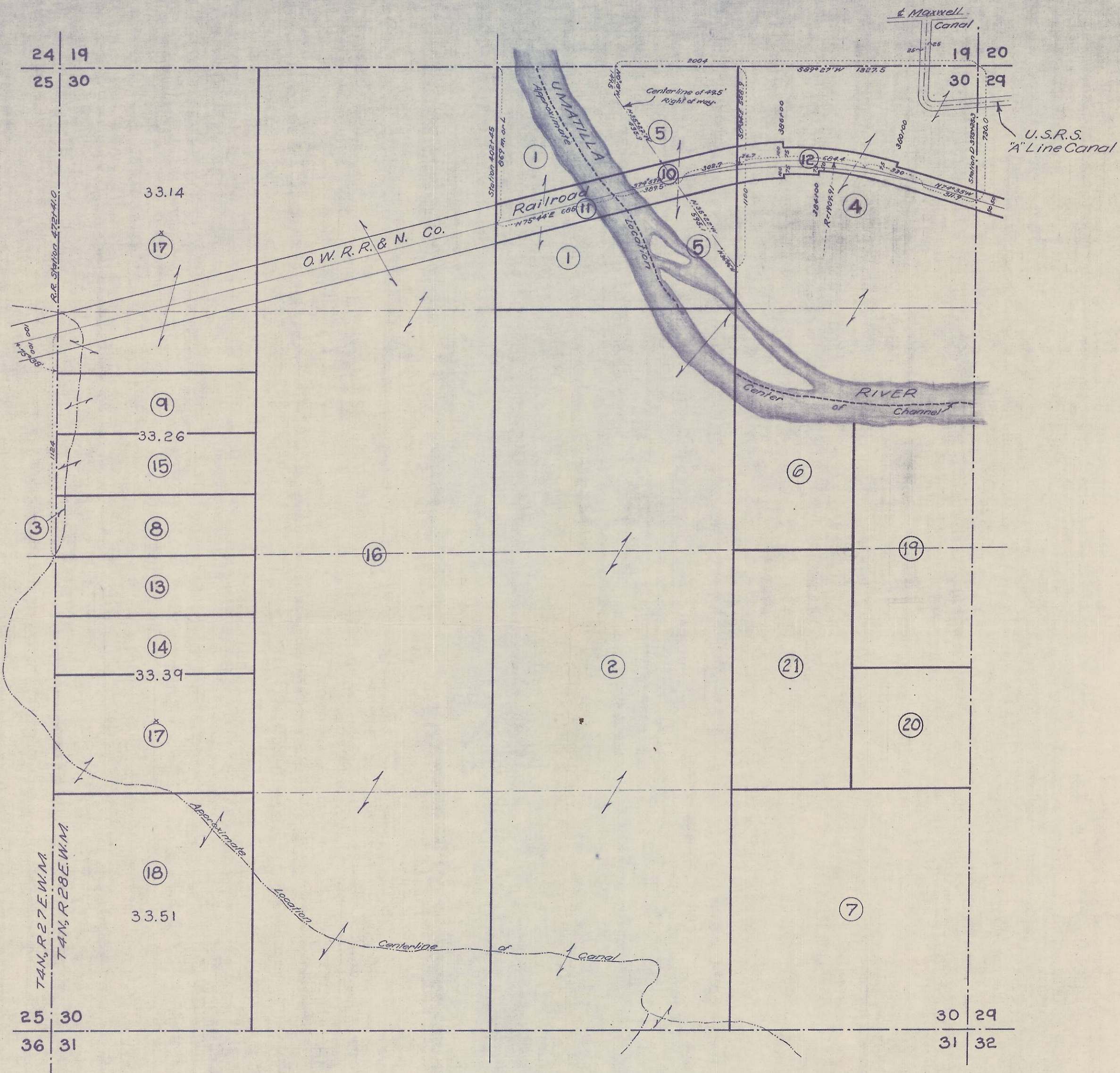
Section 30 T4N, R28E, W1M. Scale 1 inch=500 feet
